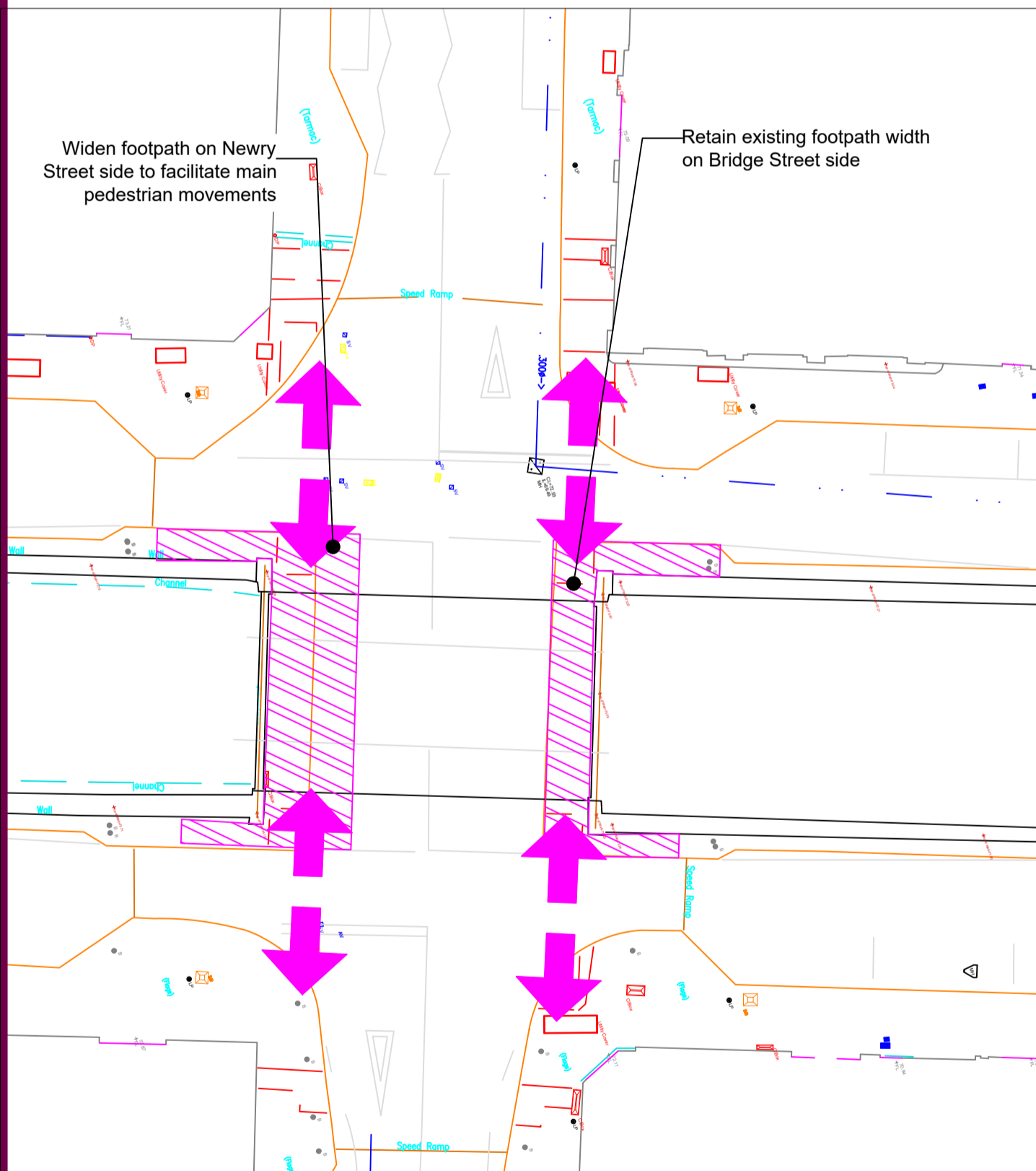
Downshire Bridge Improvements - Option 3 (Widen footpath to onside only)
