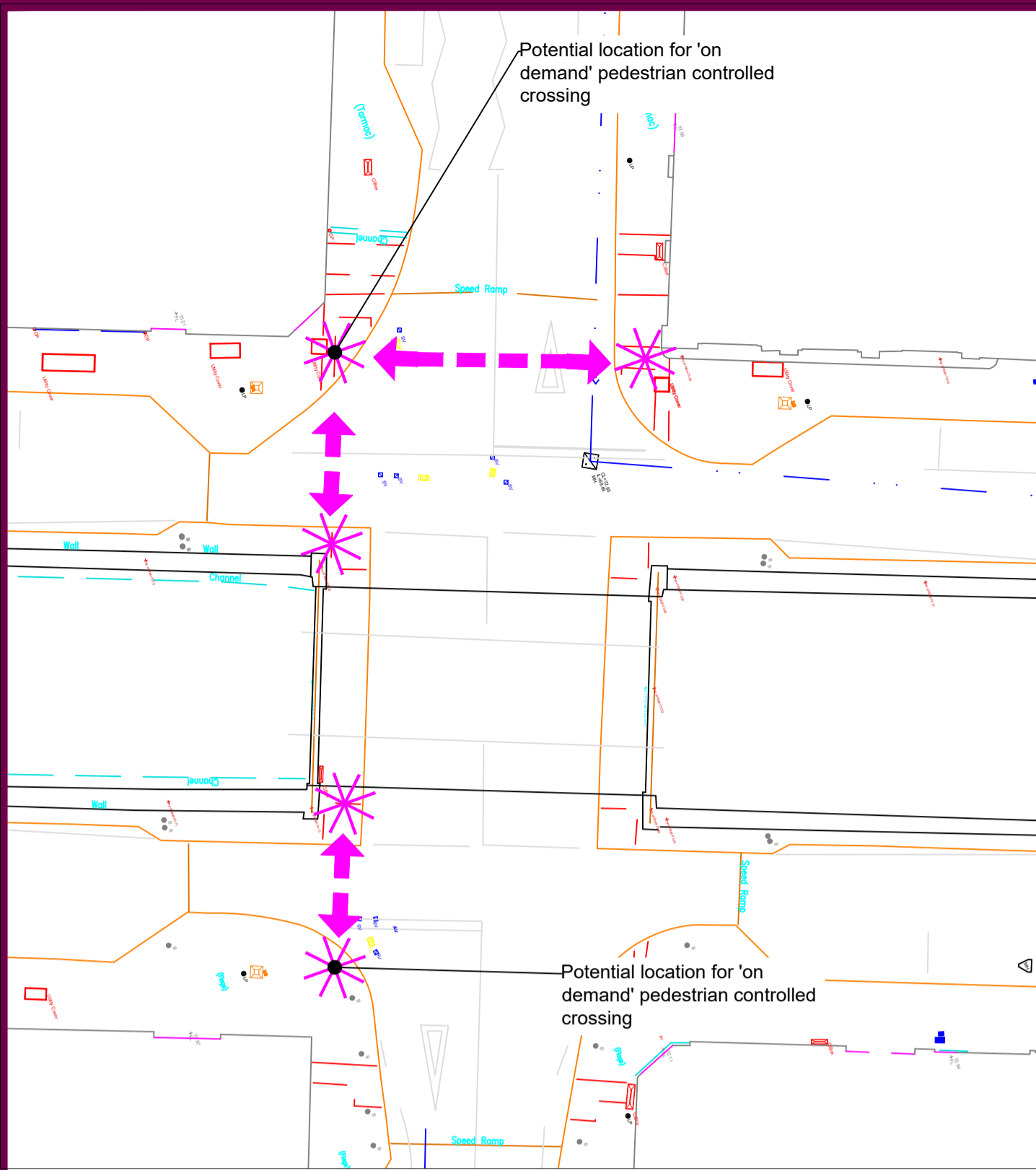
Downshire Bridge Improvements - Option 1 (Introduction of pedestrian controlled crossings)
