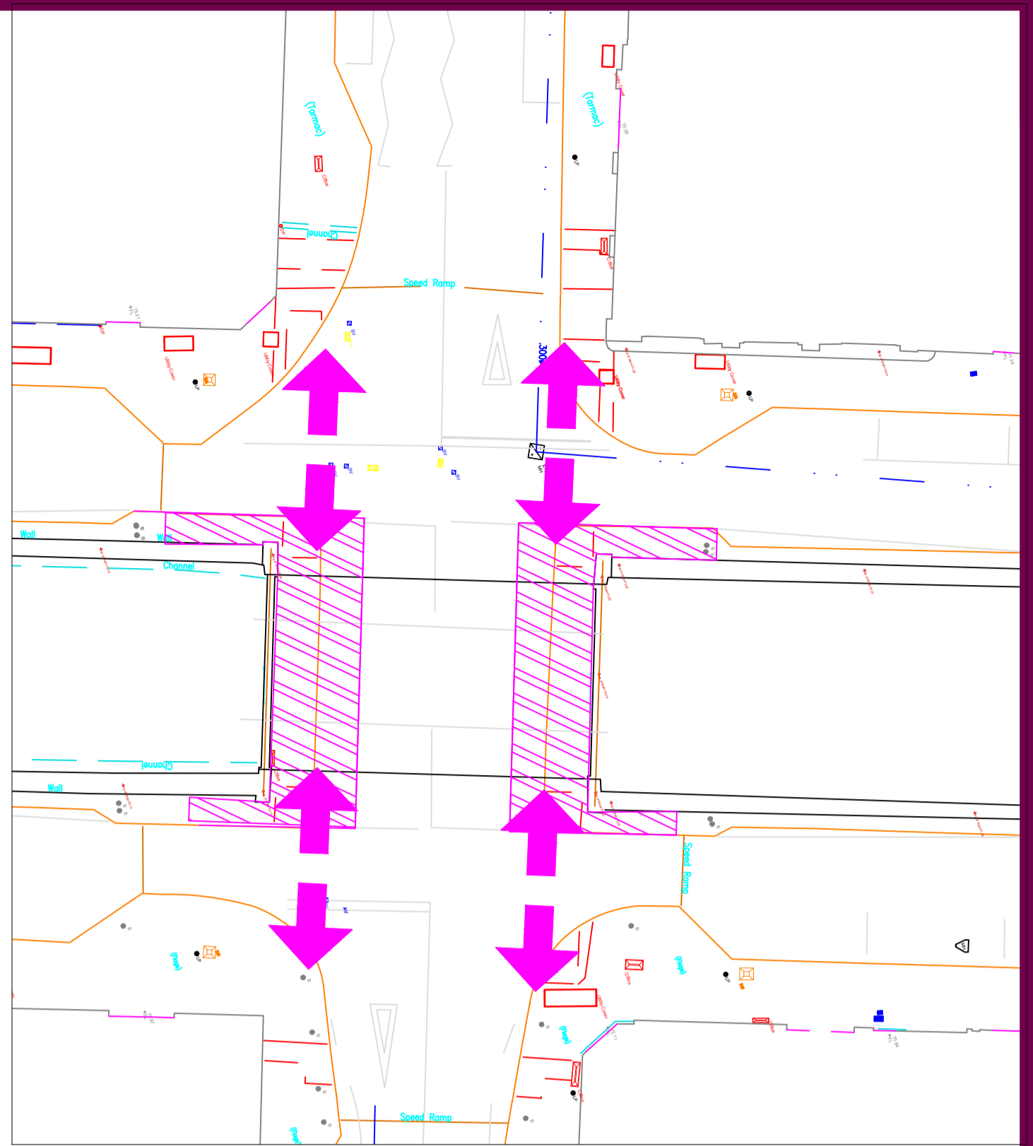
Downshire Bridge Improvements - Option 2 (Increase footways both sides and narrow carriageway)
