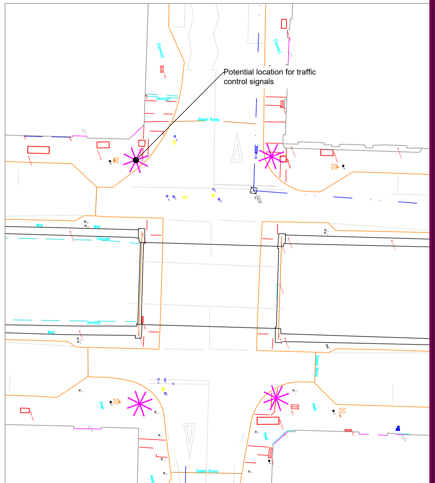
Downshire Bridge Improvements - Option 4 (Fully Signalled Junction)
